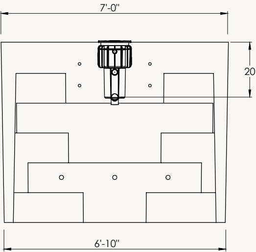
SKIMMER / STEP END VIEW
