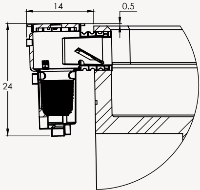
SKIMMER BOX
