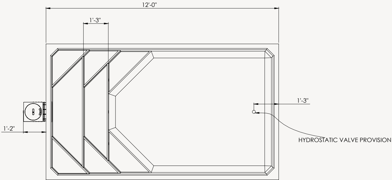
AERIAL DIMENSIONS
